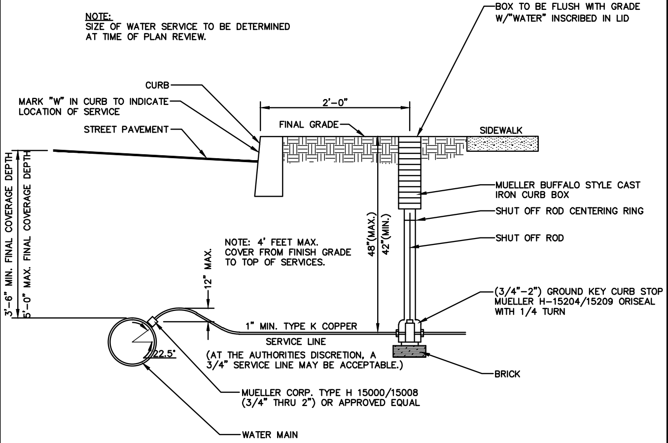
WATER SERVICE DETAIL N.T.S.
